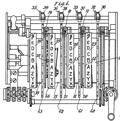
Figure 2.9: Detail of the Enigma rotors [3].
